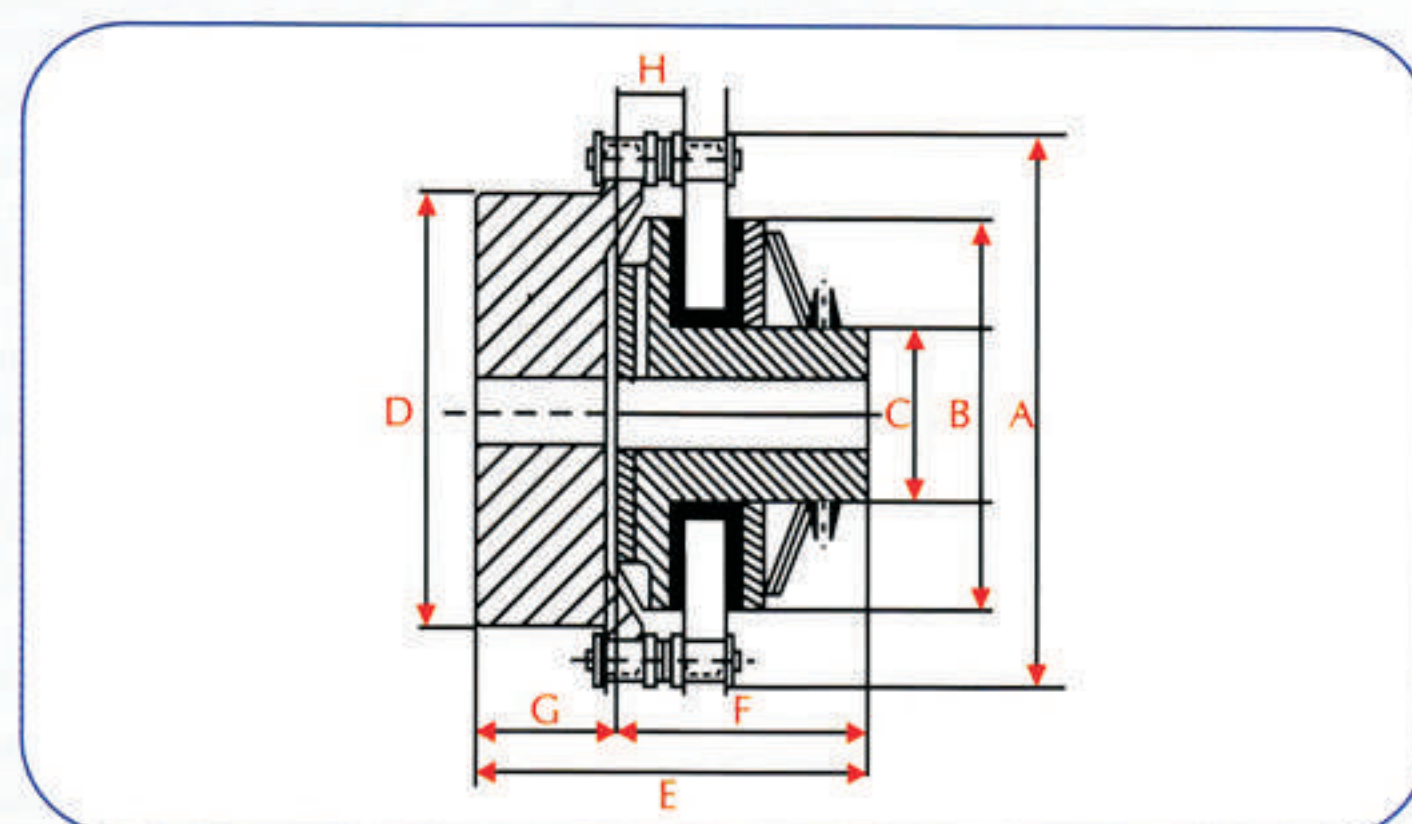
CAPACITIES & DIMENSION OF TORQUE LIMITER & COUPLINGS
